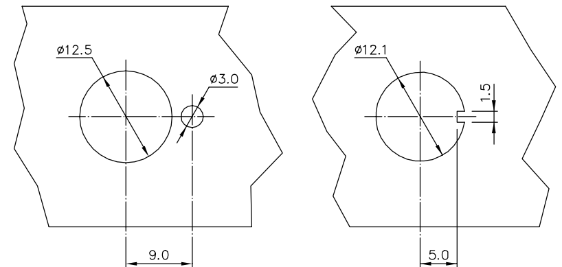
PANEL LAYOUT
