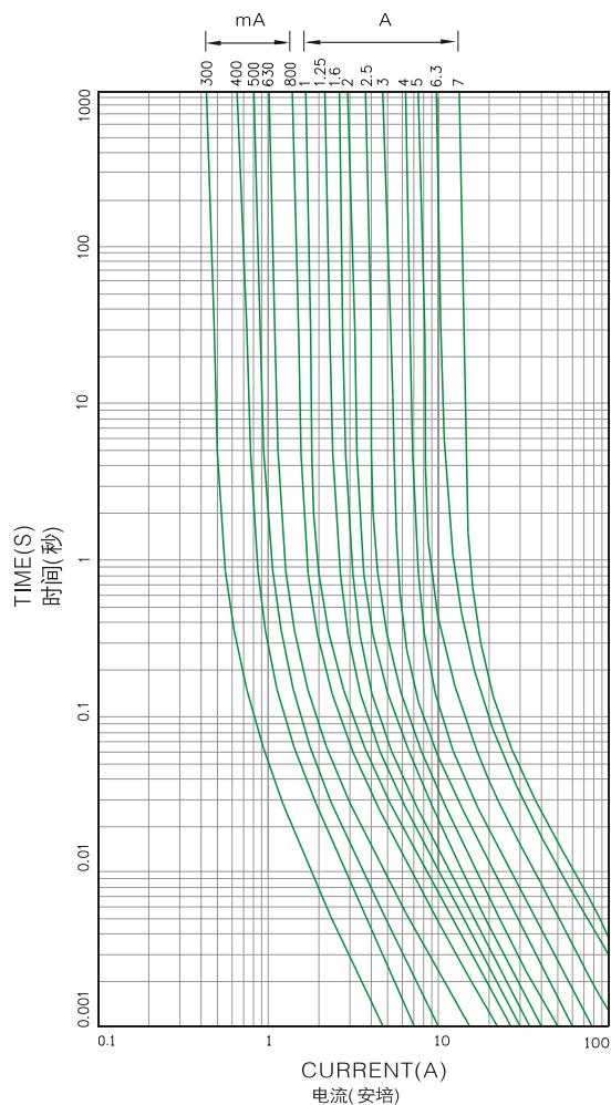
TIME-CURRENT CHARACTERISTICS 电流-时间曲线图
