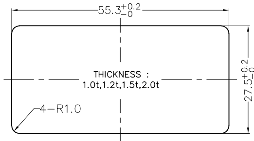
PANEL CUT-OUT
