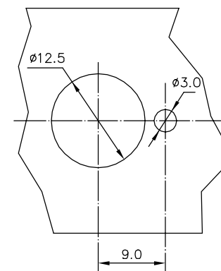
PANEL LAYOUT
