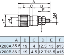
K2074 Binding post
