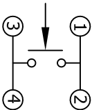
CIRCUIT
