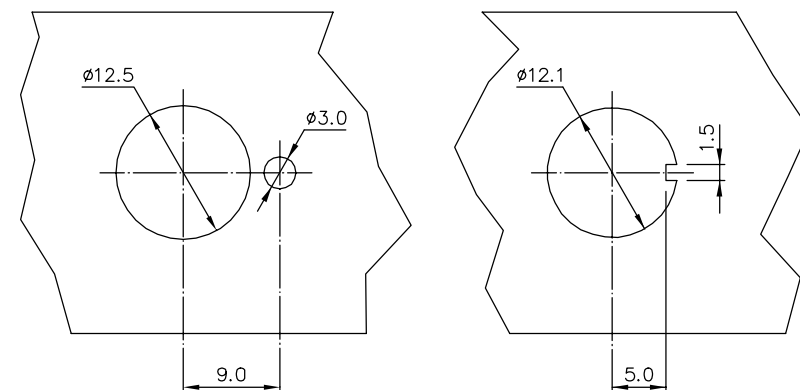
PANEL LAYOUT
