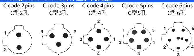
Pin assignment front view/针位分布前视图
