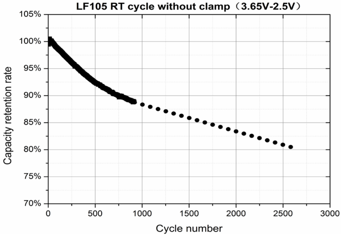
Fig.3 Cycle performance (1.0 C) curve
