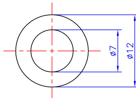
WASHER 1 PCS t=0.3
