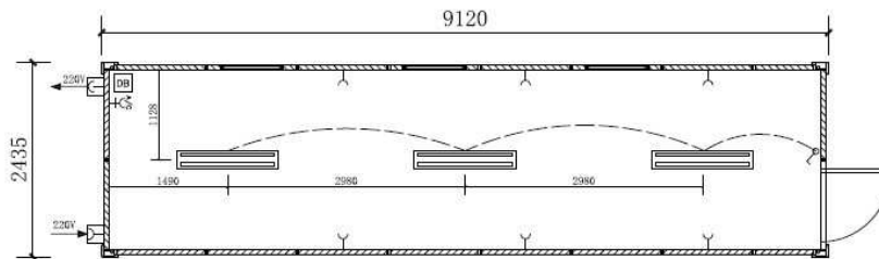
Office cabin 30'
