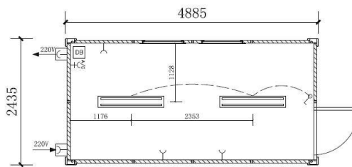
Office cabin 16'
