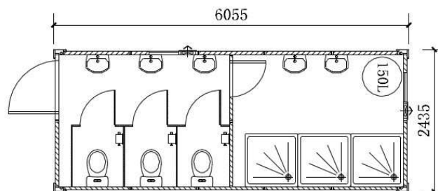
Sanitary cabin 20'
