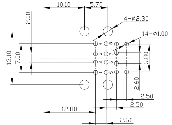
P.C.B LAYOUT BOTTOM VIEW P.C.B Tolerance ±0.1
