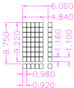
DETAIL DOTS
