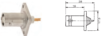
M5543T BNC female chassis mount gold-pin teflon insulation
