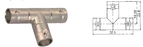
M5551 T-type BNC male to double BNC female gold-pin
