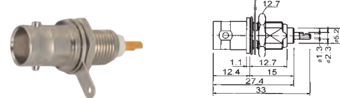
M557740 BNC female bulkhead long thread gold-pin
