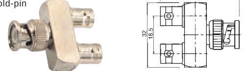
M55793 Right angle BNC male to double BNC female gold-pin
