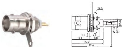
M5542 BNC female bulkhead gold-pin
