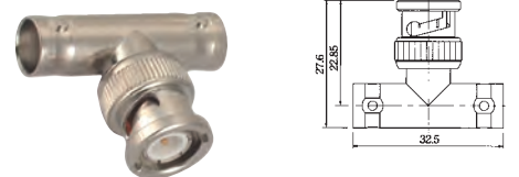
M5551 T-type BNC male to double BNC female gold-pin
