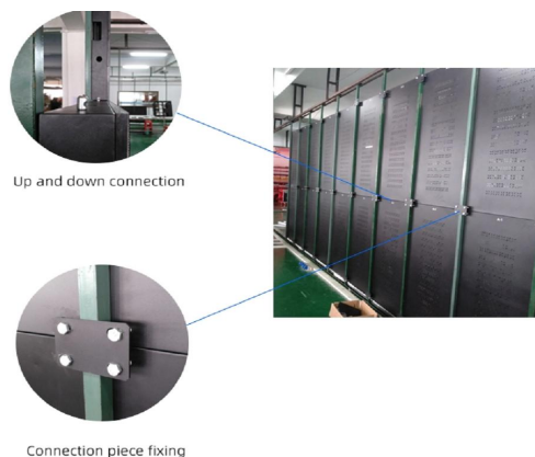
Connection piece fixing
