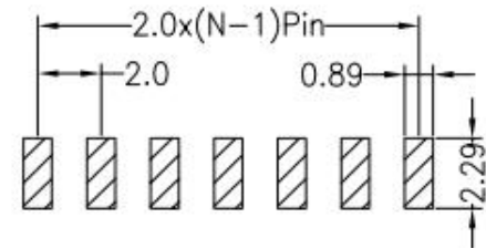
Recommended P.C.B Layout(Top Side) (PCB BOARD TOLERANCE±0.05)
