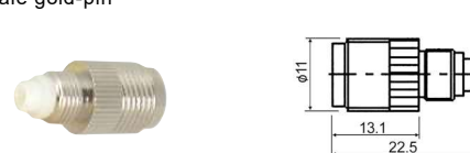
M57766 FME female to TNC female gold-pin
