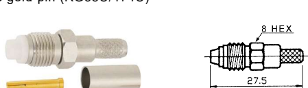
M577501 FME female crimp type gold-pin (RG58U/174U)
