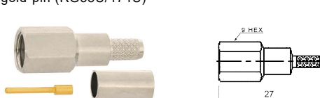
M577502 FME male crimp type gold-pin (RG58U/174U)
