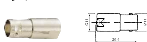
M57771 FME male to BNC female gold-pin
