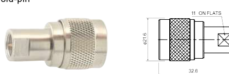
M57753 FME male to mini UHF male gold-pin
