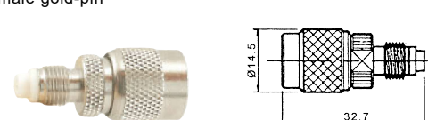
M57767 FME female to TNC male gold-pin
