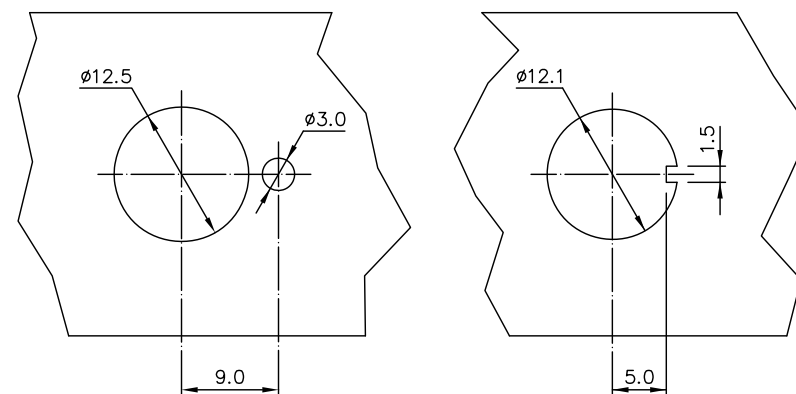
PANEL LAYOUT
