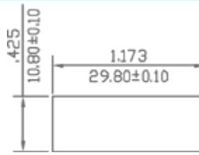
Mounting Hole of Snap-in Type
