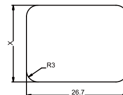
PANEL CUT-OUT
