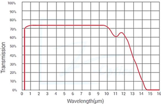
ZnS Transmission
