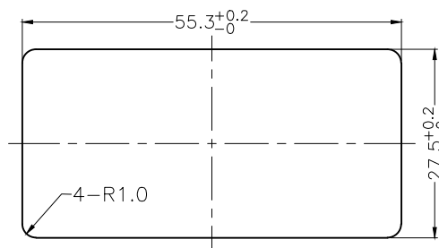
PANEL CUT-OUT
