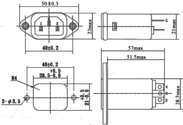
Standard case drawing
