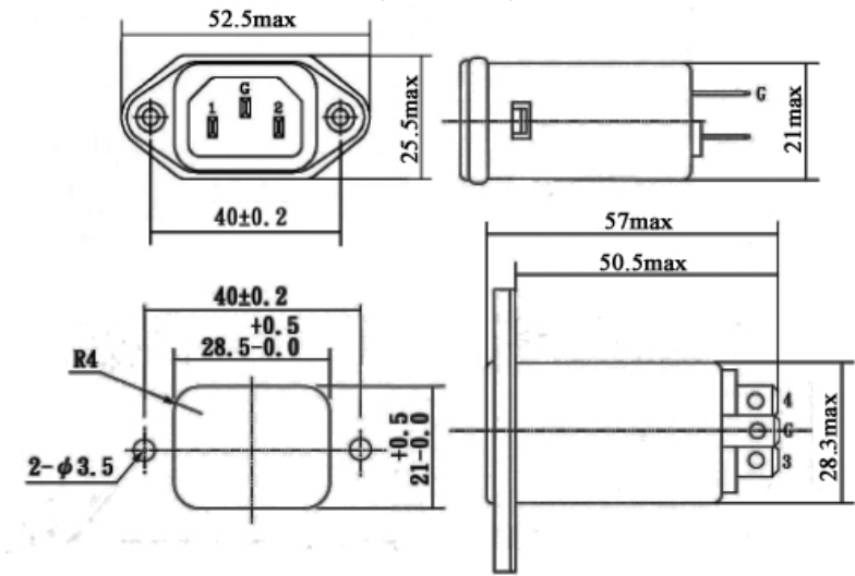
Big case drawing
