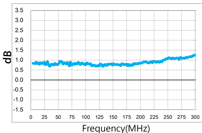
Amplitude Balance
