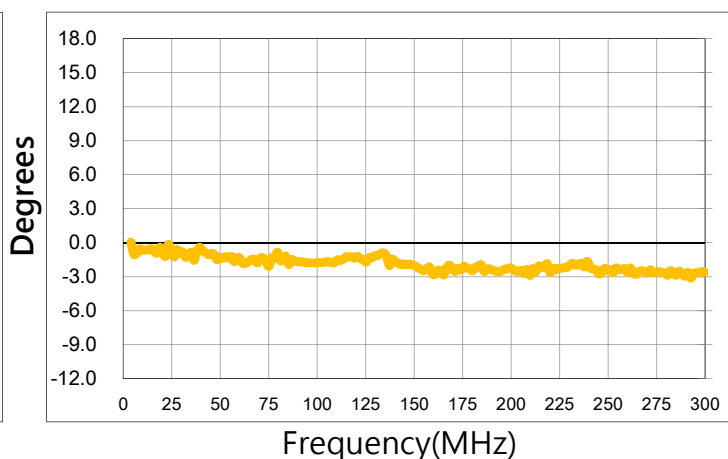
Phase Balance
