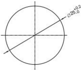
Panel Cutout Ø25 mm (Panel thickness : 7 mm MAX)
