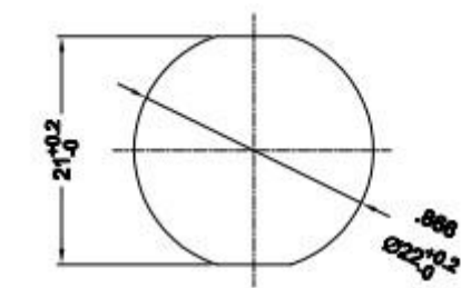
Panel Cutout Ø22 mm (Panel thickness : 3.5 mm MAX)
