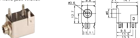
K3634 3.5mm Stereo phone jack
