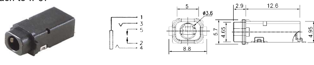
K36440 Waterproof 3.5mm stereo phone jack (SMD) can reach to IP67
