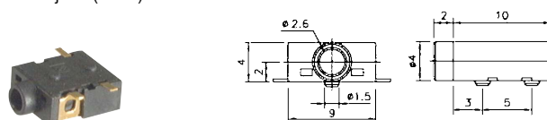
K36400A /B /C /D /E 2.5mm Phone jack (SMD)
