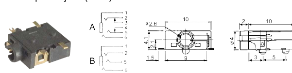
K36404A /C /E 2.5mm Phone jack (SMD)
