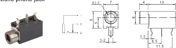
K3633A /B /C /D /E 3.5mm Phone jack W/shell
