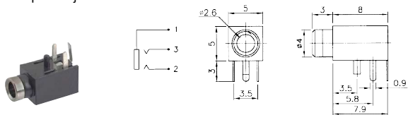
K3625 2.5mm Stereo phone jack
