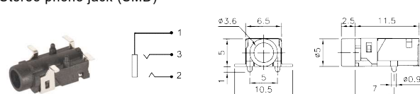
K36406 3.5mm Stereo phone jack (SMD)
