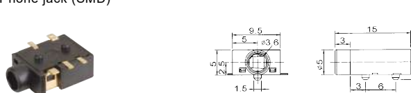
K36411A /B /C /D /E 3.5mm Phone jack (SMD)
