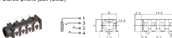
K36420 3.5mm Stereo phone jack (SMD)
