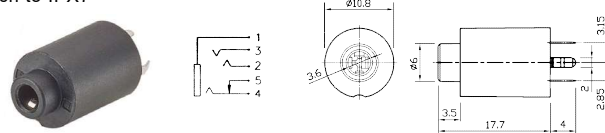
K36380 Waterproof 3.5mm stereo phone jack can reach to IPX7
