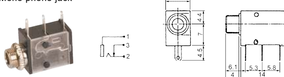
K3630 3.5mm Mono phone jack
