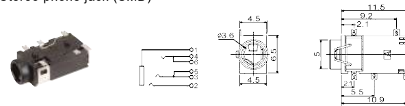
K36420 3.5mm Stereo phone jack (SMD)
