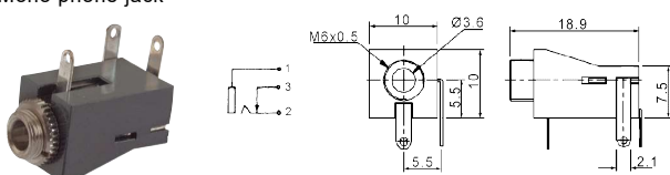
K3632 3.5mm Mono phone jack
