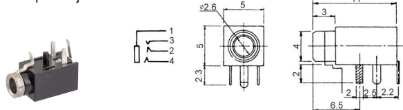
K3626 3.5mm Mono phone jack
