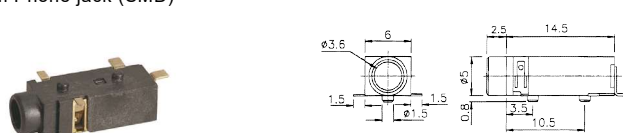
K36414A /C /D /E 3.5mm Phone jack (SMD)
