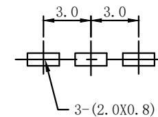
P.C.B LAYOUT TOP VIEW
