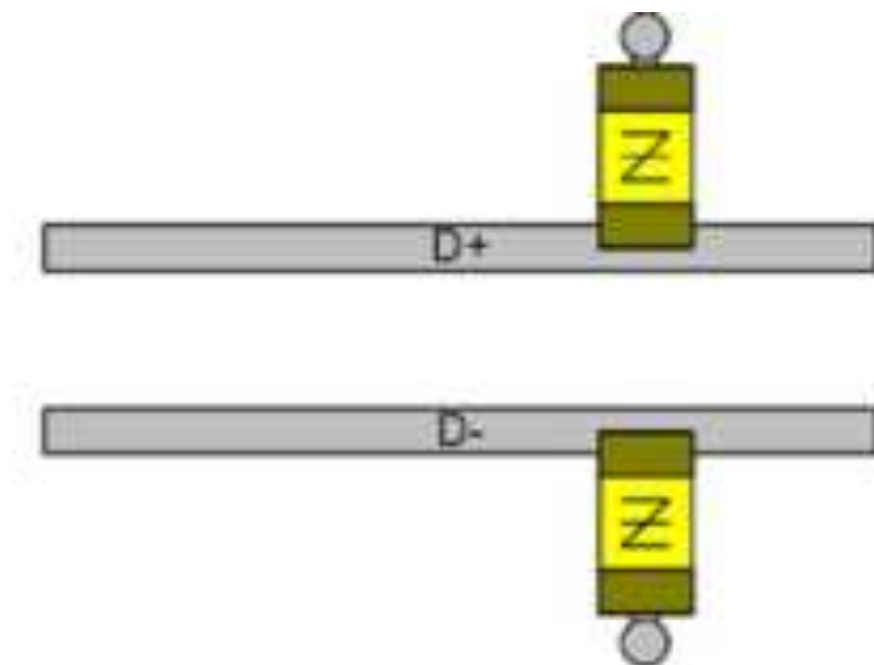
Fig.3-4 RK3126C USB OTG/Host2.0 component placement.
