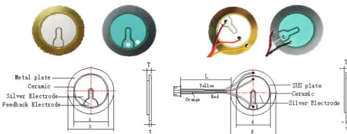
产品和尺寸示意图 Product Image and dimension drawing
