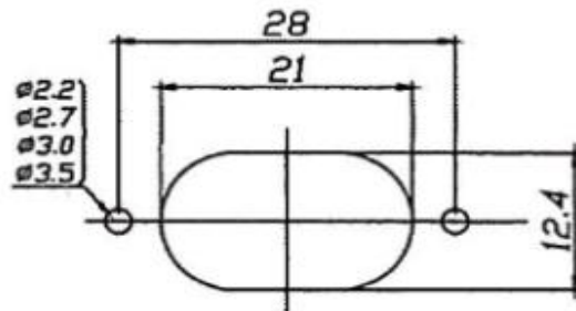
PANEL CUT-OUT
