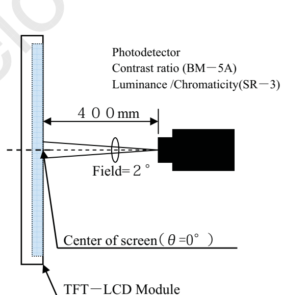
Fig3-2 Luminance/Contrast ratio/Response time/Chromaticity measurement method
