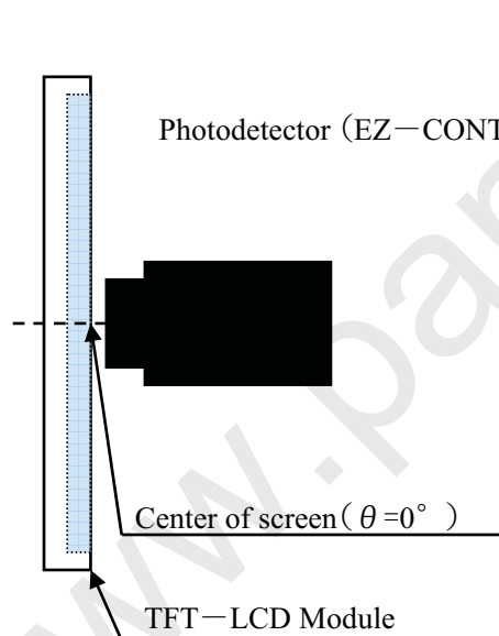
Fig3-1 Viewing angle measurement method
