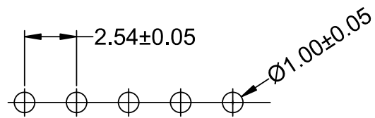
Recommended P.C.B Layout General Tolerance±0.05
