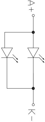
LED CIRCUIT:
