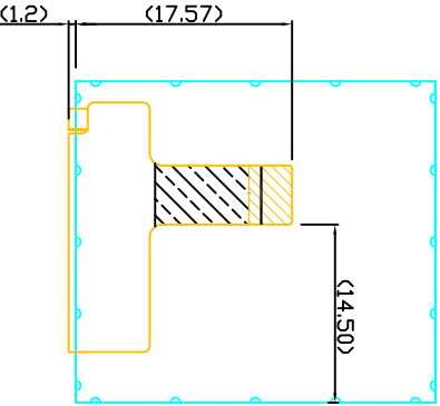
FPC bending diagram
