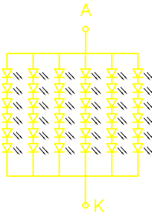
Backlight LED Circuit If=120mA,Vf=18-20V
