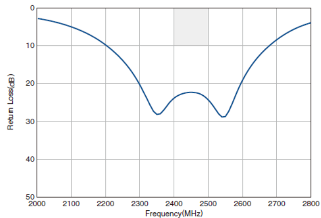
□ RETURN LOSS
