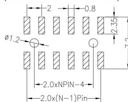
Recommended P.C.B Layout(Top Side) (PCB BOARD TOLERANCE±0.05)
