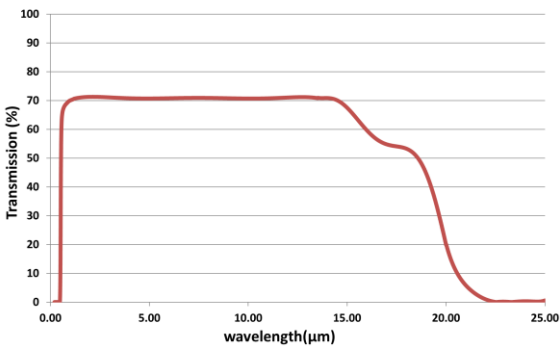
ZnSe Transmission
