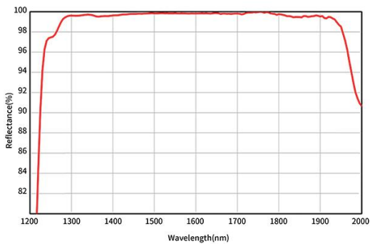
D04 Coating 0° AOI @ 1200 ~ 1800nm
