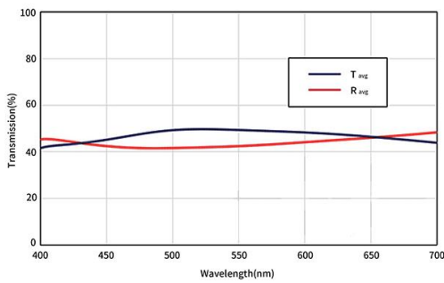
VIS Non-Polarizing Beamsplitters(50R/50T)
