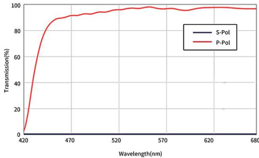
Polarizing Beamsplitter 420 ~ 680nm Coating
