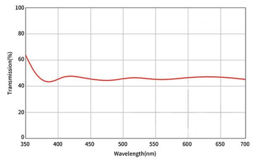
VIS 50R/50T Transmitted
