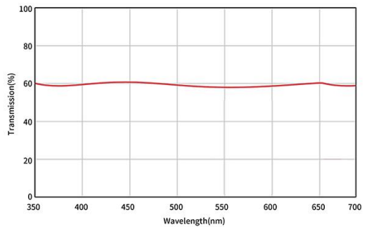
VIS 40R/60T Transmitted
