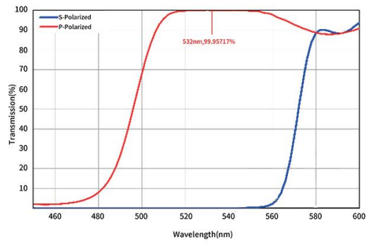
Polarizing Beam splitter 532nm Coating
