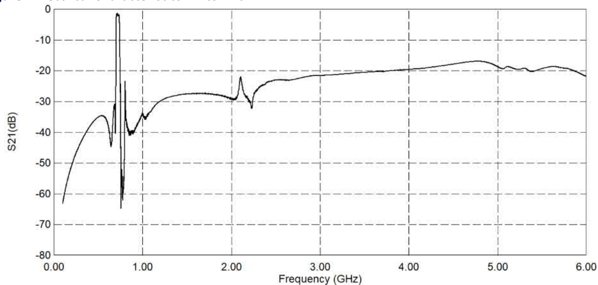
Figure 2 Electrical Characteristics: Tx to Ant.
