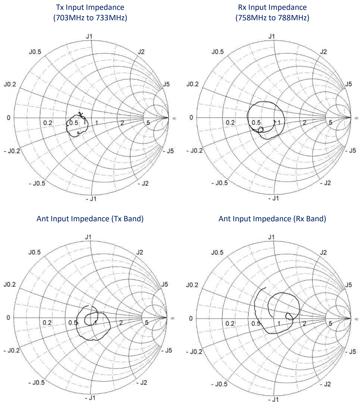
Figure 7 Input Impedances.
