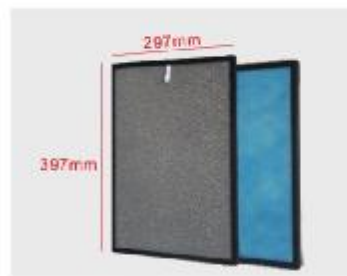
Filter size
