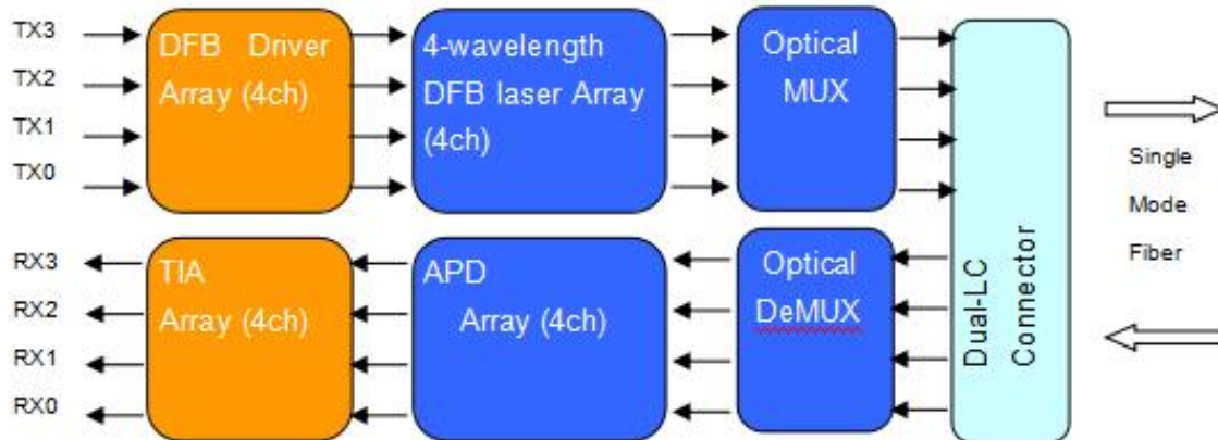
Figure 1: 40Gb/s QSFP ER4 Transceiver Block Diagram
