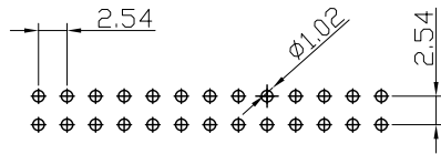
PCB LAYOUT
