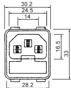
K2414 Panel mount AC socket terminal 4.8mm
