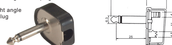
K303K 1/4" Right angle mono plug
