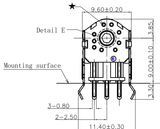
Detail E(1:1) Shaft hole shape and dimension
