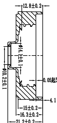
SECTION B-B
