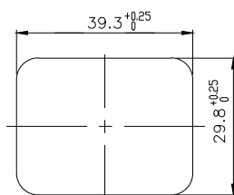
PANEL CUTOUT
