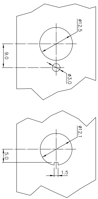
PANEL LAYOUT
