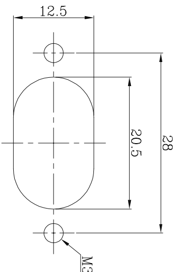
PANEL CUT-OUT
