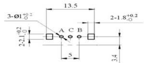
Mounting hole detail
