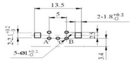
Mounting hole detail
